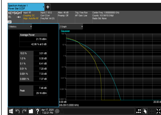
Band2-5MHz-16QAM-18900-1RB#0-PASS
