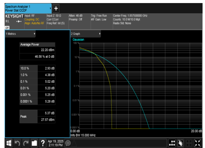
Band2-15MHz-16QAM-18675-1RB#0-PASS
