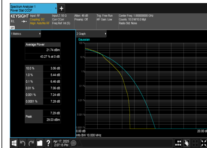
Band2-10MHz-16QAM-18900-1RB#0-PASS
