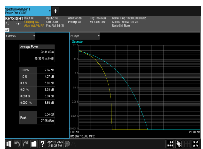
Band2-15MHz-QPSK-18900-1RB#0-PASS
