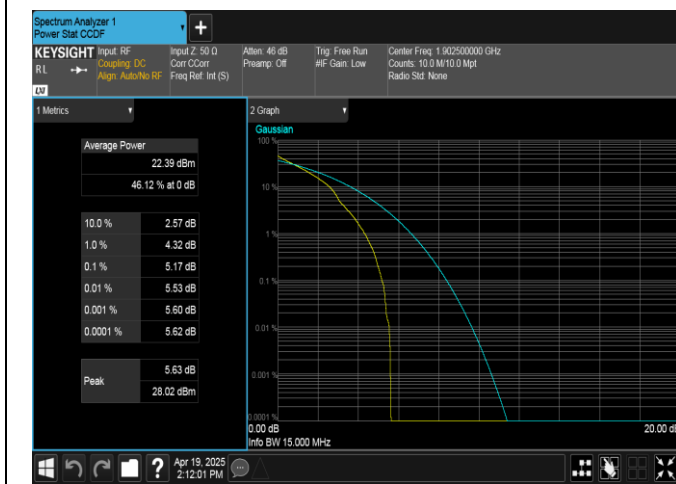
Band2-15MHz-QPSK-19125-1RB#0-PASS
