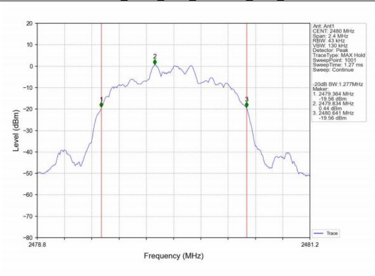
Pi/4DQPSK_2DH5_HCH_2480MHz_Ant1_NTNV
