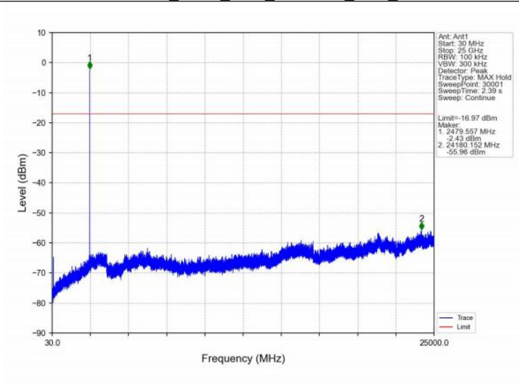
Pi/4DQPSK_2DH5_HCH_2480MHz_Ant1_NTNV
