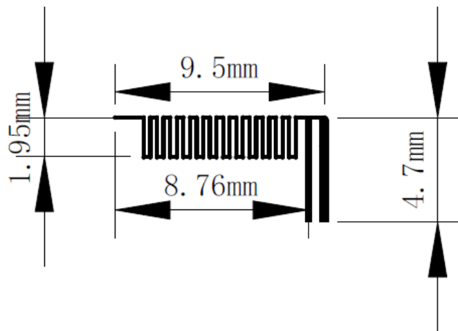
Antenna Dimensions
