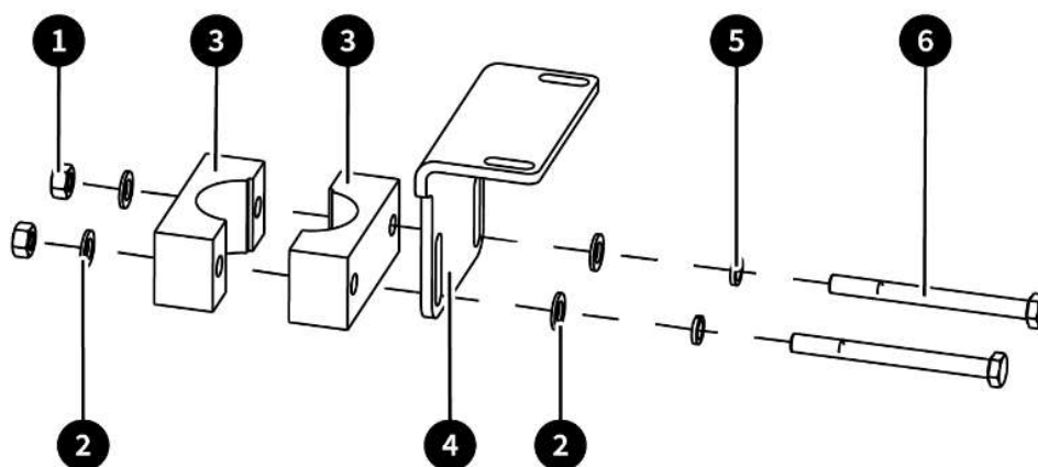
2# Motor Bracket (Component 7 of the Electric Steering Wheel Assembly)
