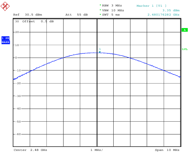
BLE_1M_High_Channel
