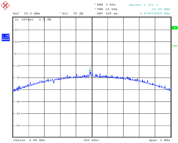
BLE_2M_High_Channel
