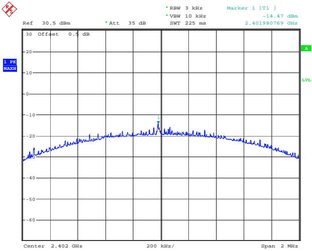
BLE_2M_Low_Channel
