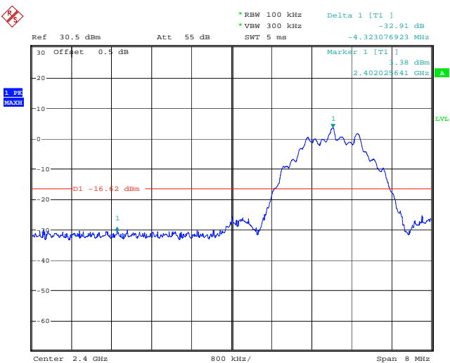
BLE_2M_Low_Channel
