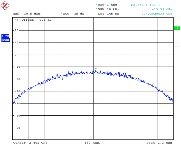
BLE_1M_Low_Channel
