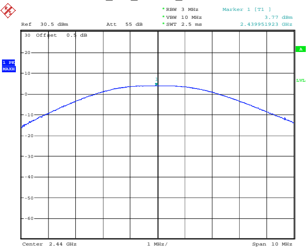
BLE_2M_Middle_Channel
