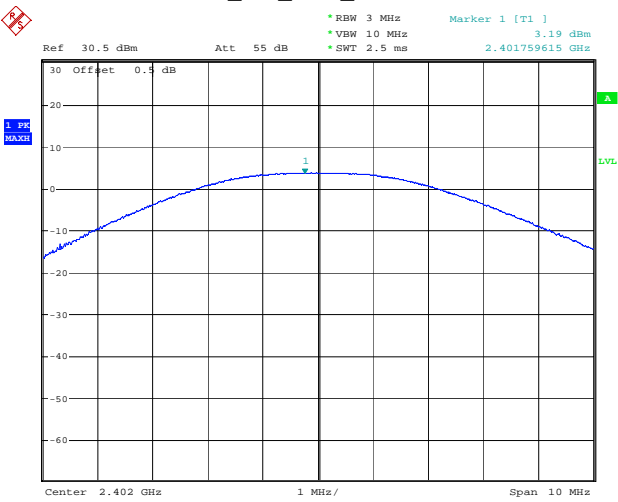
BLE_2M_Low_Channel
