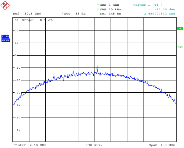
BLE_1M_High_Channel
