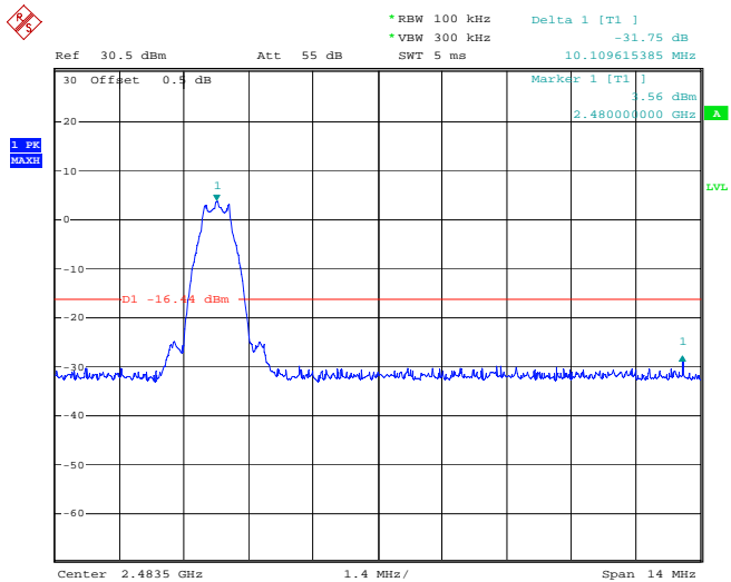
BLE_1M_High_Channel
