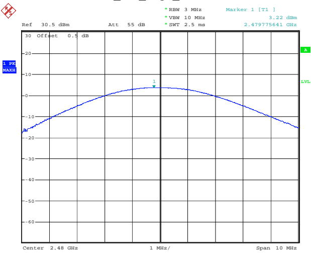
BLE_2M_High_Channel
