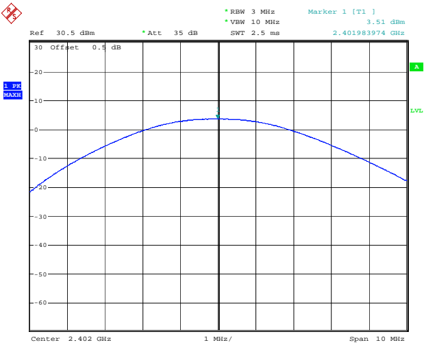
BLE_1M_Low_Channel
