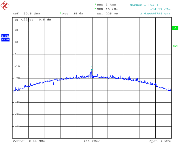
BLE_2M_Middle_Channel
