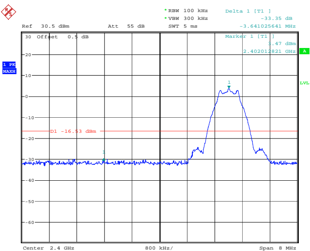
BLE_1M_Low_Channel
