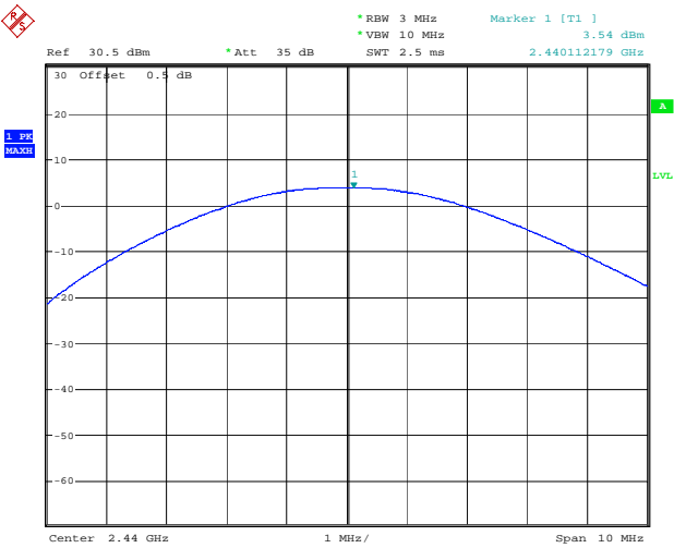
BLE_1M_Middle_Channel
