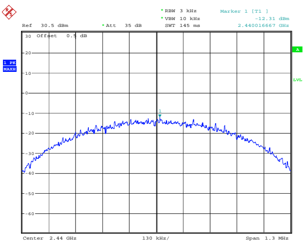
BLE_1M_Middle_Channel
