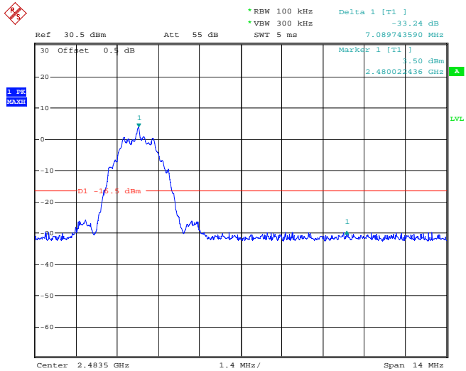
BLE_2M_High_Channel
