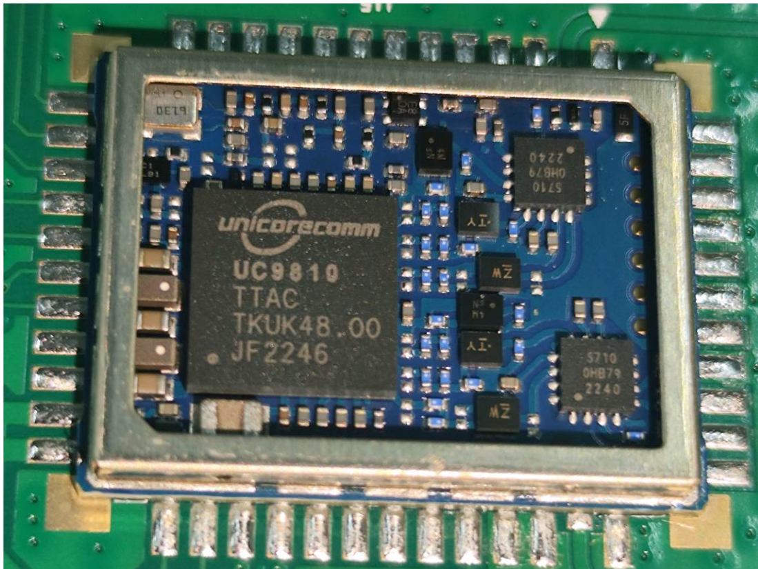
GNSS Module Unshielded
