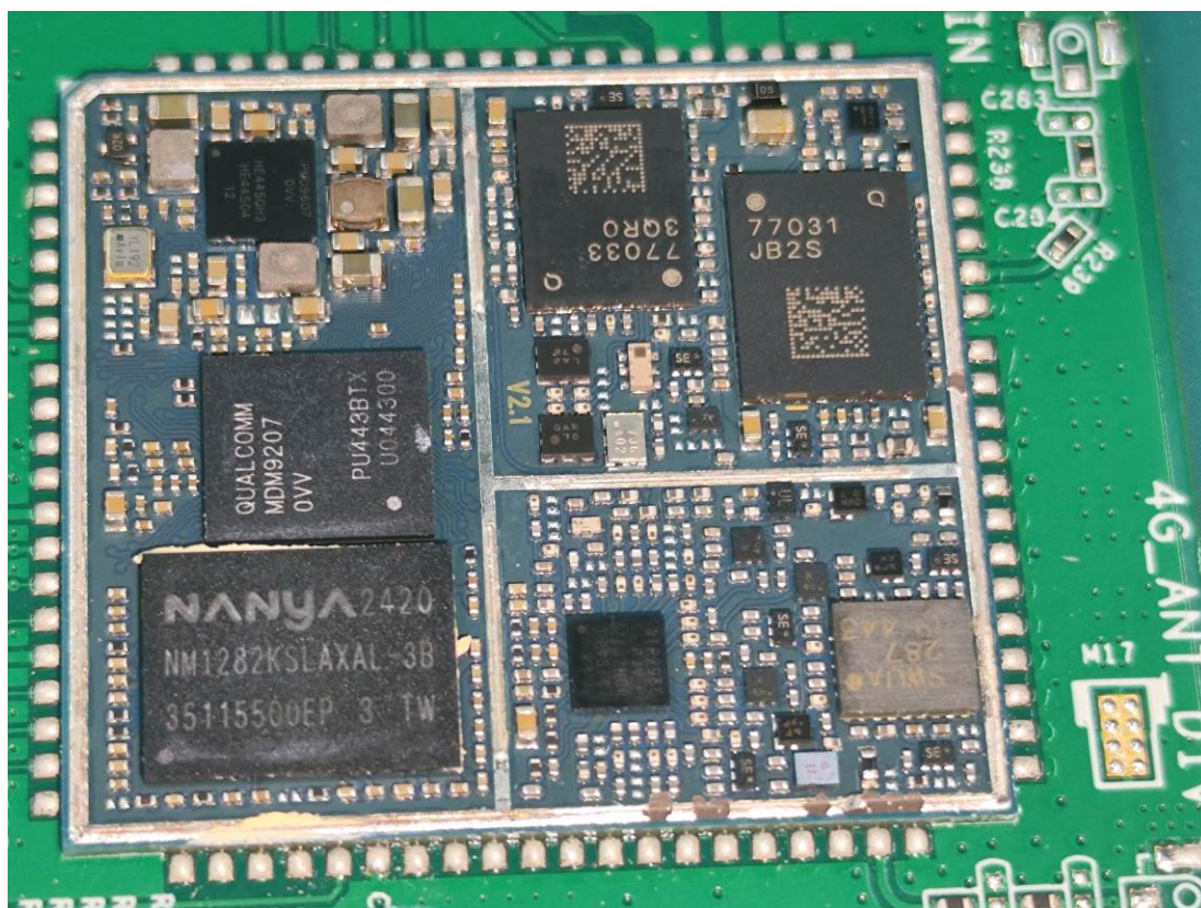
WWAN Module Unshielded
