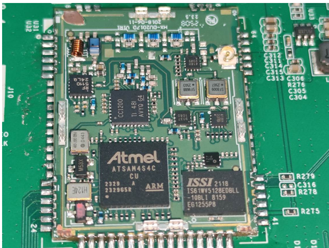
900MHz Module (only RX) Unshielded
