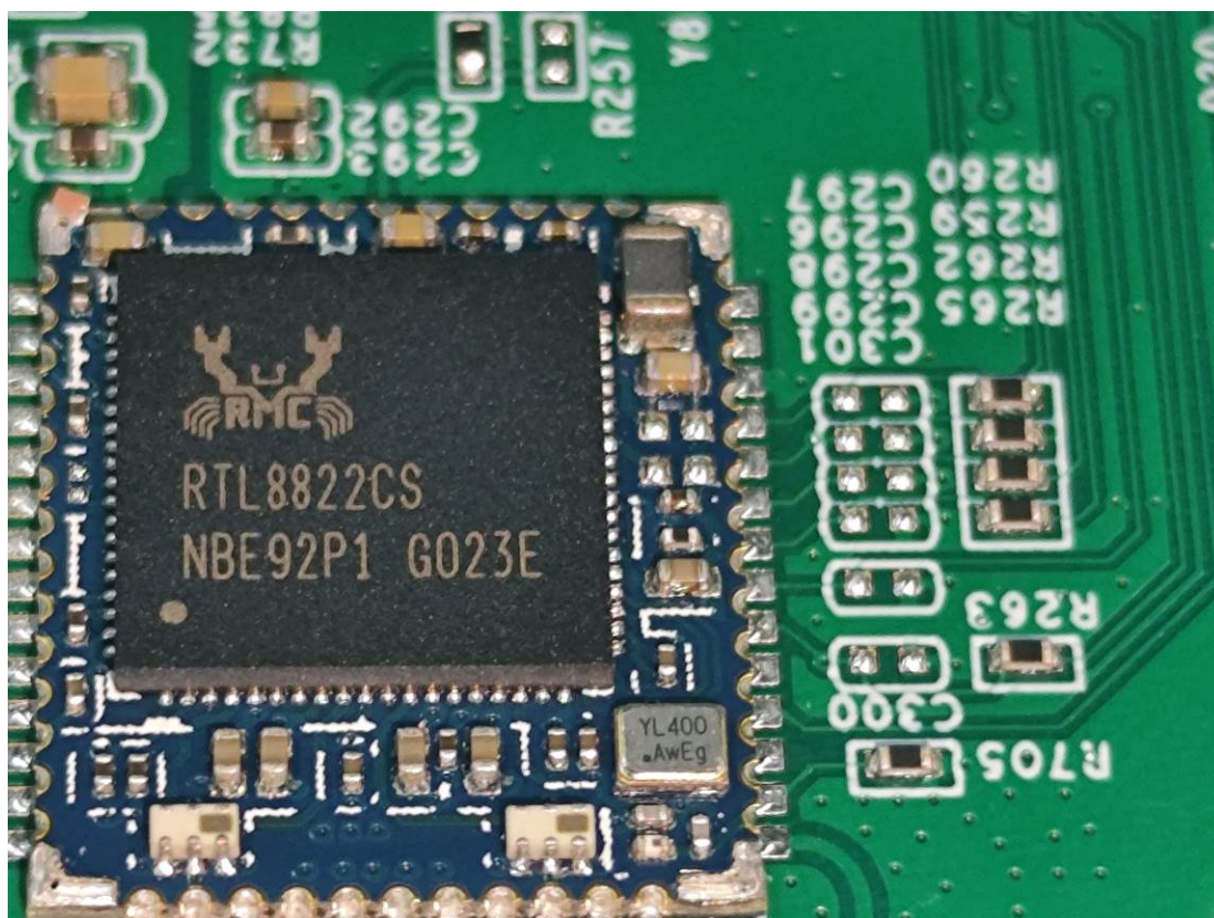
Wi-Fi&Bluetooth Module Unshielded
