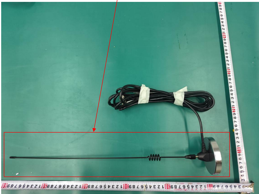
Radio Antenna (With Coaxial Harness)
