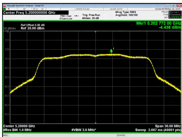
(802.11ax20) PSD plot on channel 40
