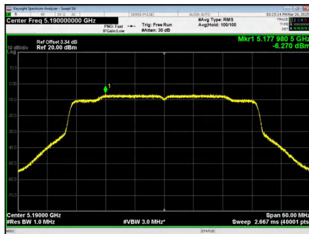
(802.11ax40) PSD plot on channel 38
