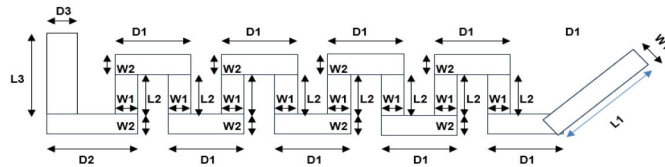
Antenna Dimensions
