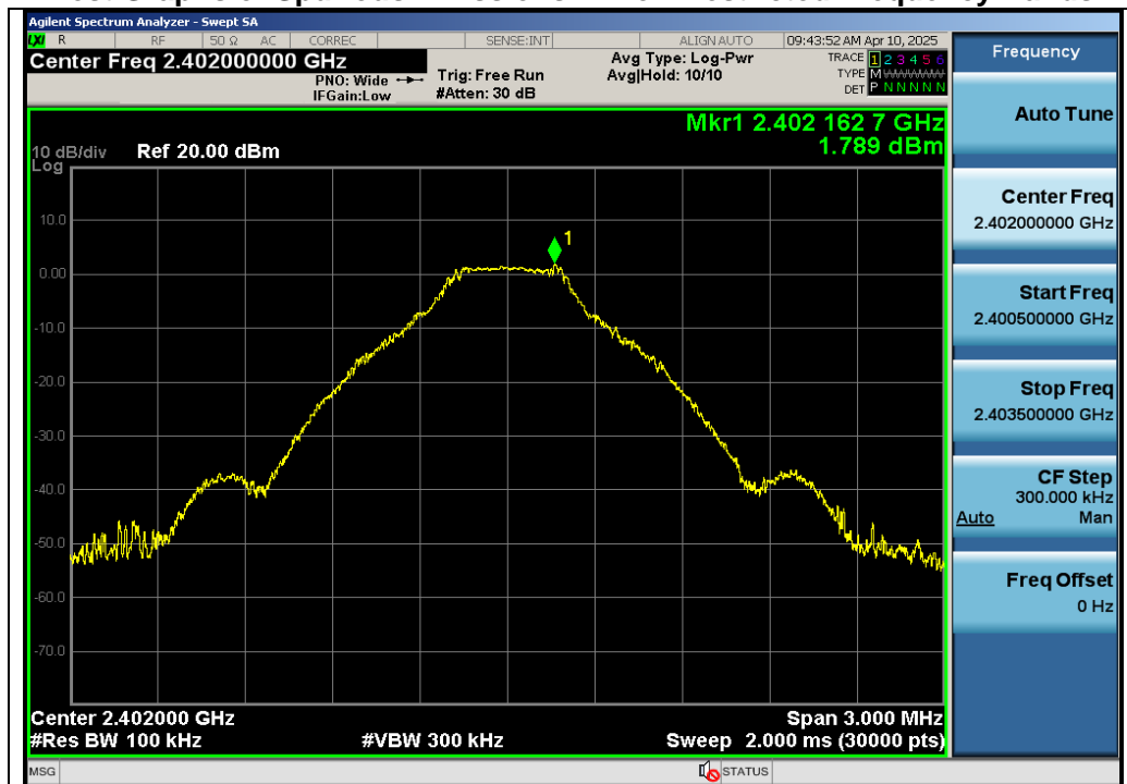
Test_Graph_BR_ANT1_2402_1Mbps_Reference Level
