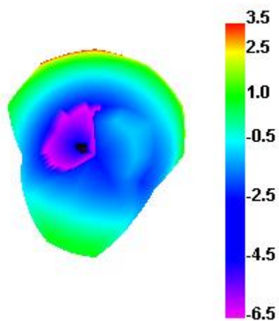
Bluetooth 78 TRP
