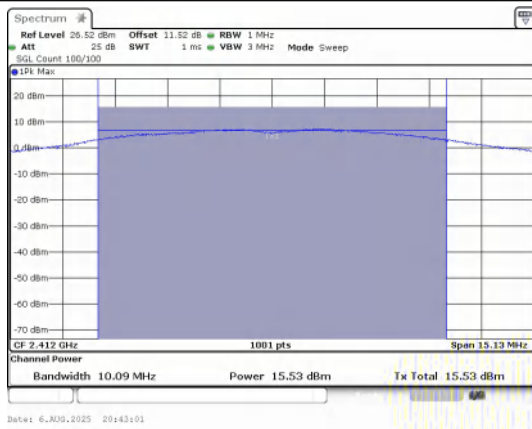
Conducted Output Power IEEE 802.11n_Channel 1_Antenna 0
