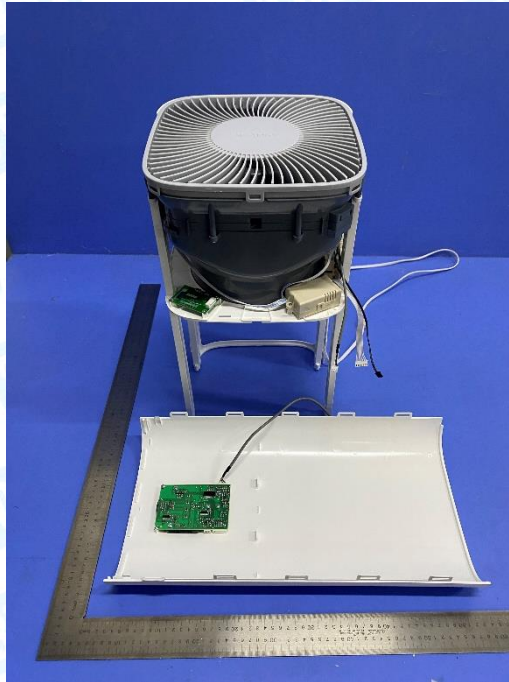
Photo 9 Internal of EUT
