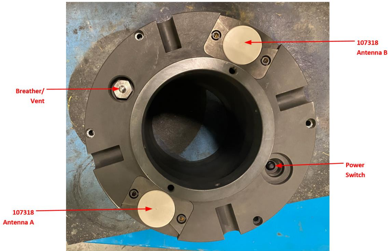
Bottom View:
