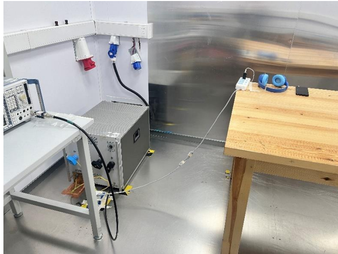
Radiated Emission
