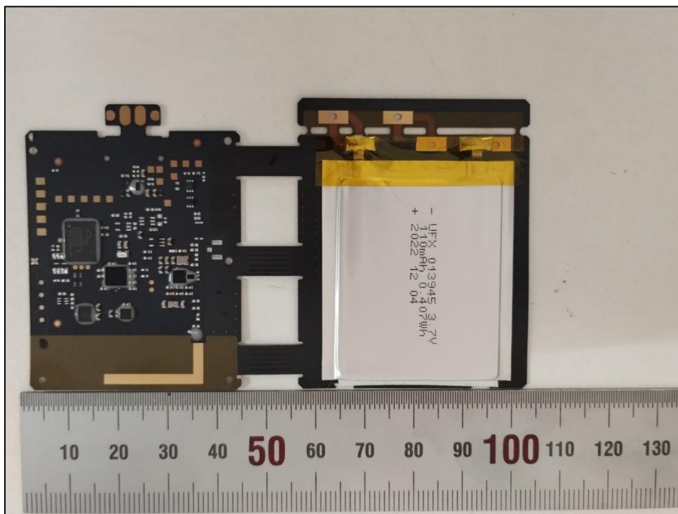
Figure 3: Dimensional view of PCB
