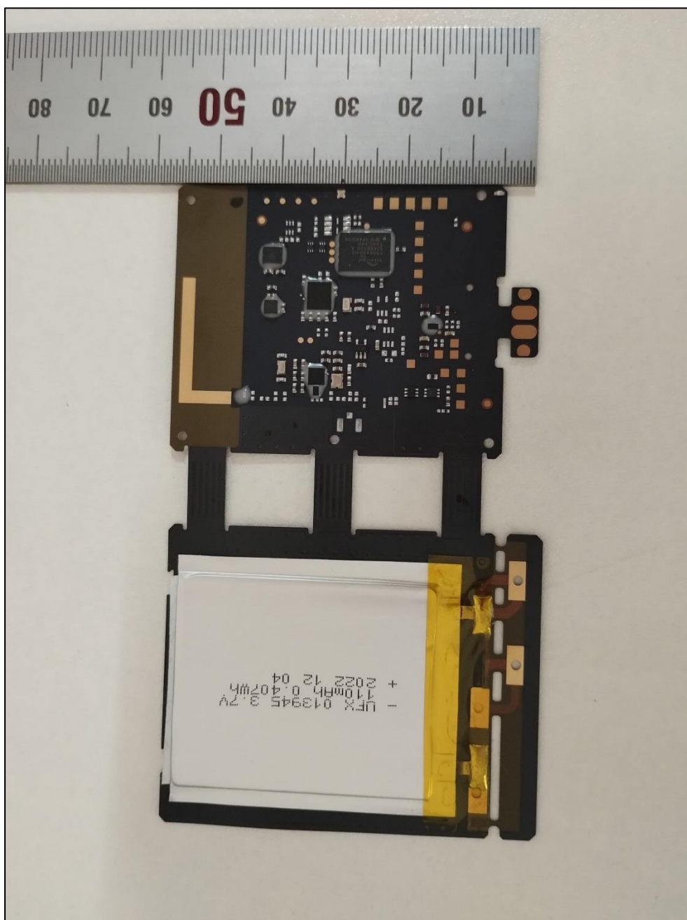
Figure 2: Dimensional view of PCB
