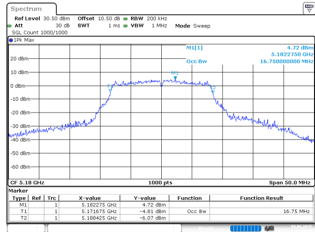
802.11a_5180MHz_Chain 0
