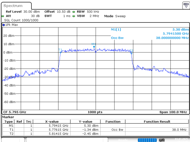
802.11ax40_5795MHz_Chain 0
