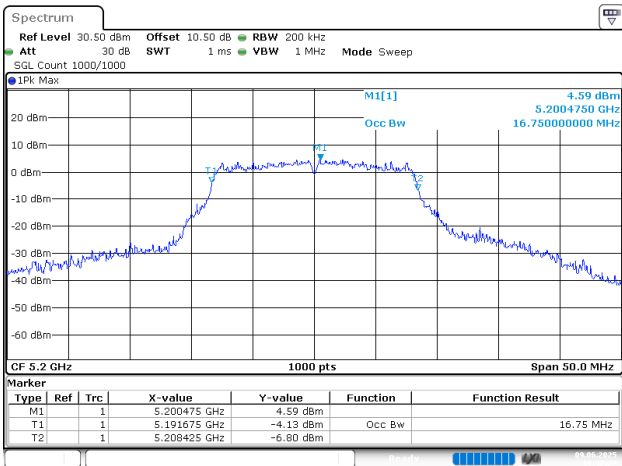
802.11a_5200MHz_Chain 0
