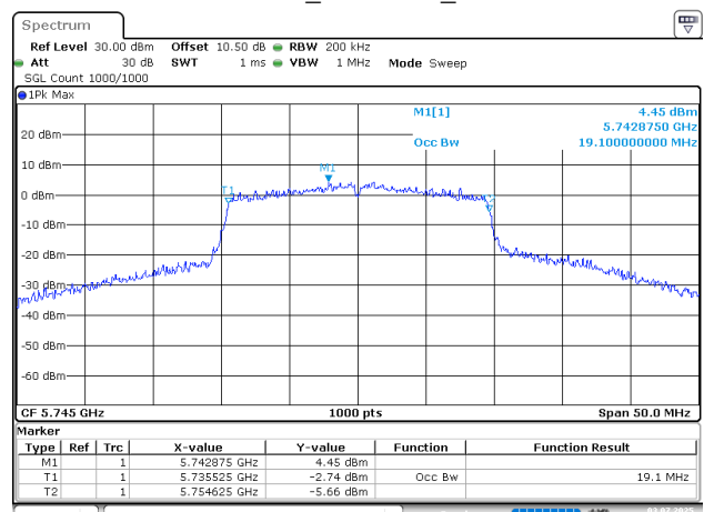
802.11ax20_5745MHz_Chain 0
