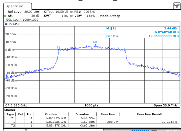
802.11ax20_5825MHz_Chain 0
