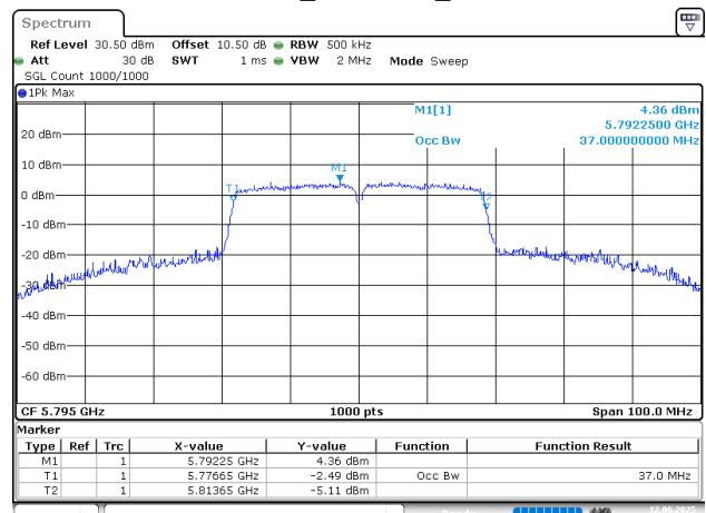
802.11n40_5795MHz_Chain 0
