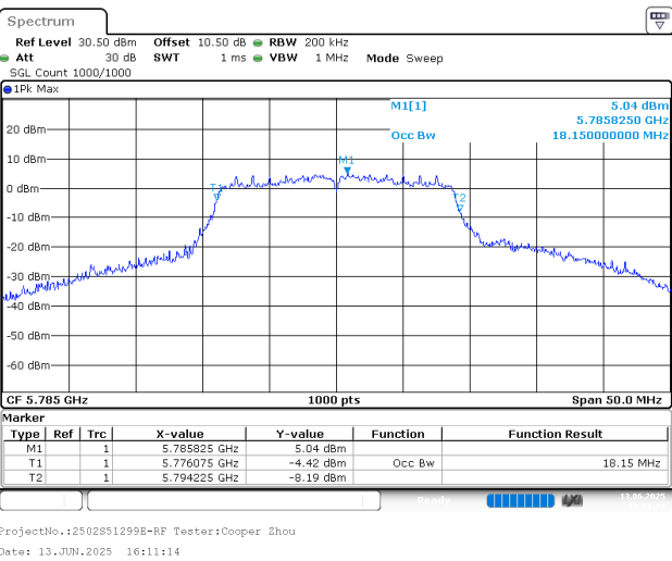
802.11n20_5785MHz_Chain 0
