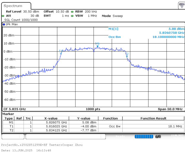
802.11n20_5825MHz_Chain 0
