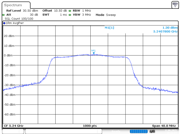
802.11n20_5240MHz_Chain 1
