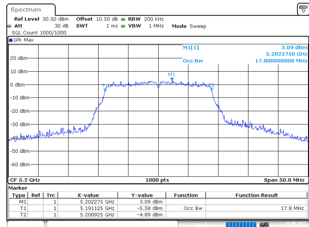
802.11n20_5200MHz_Chain 0
