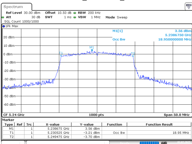
802.11ax20_5240MHz_Chain 0
