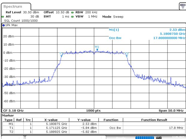
802.11n20_5180MHz_Chain 0
