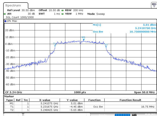
802.11a_5240MHz_Chain 0
