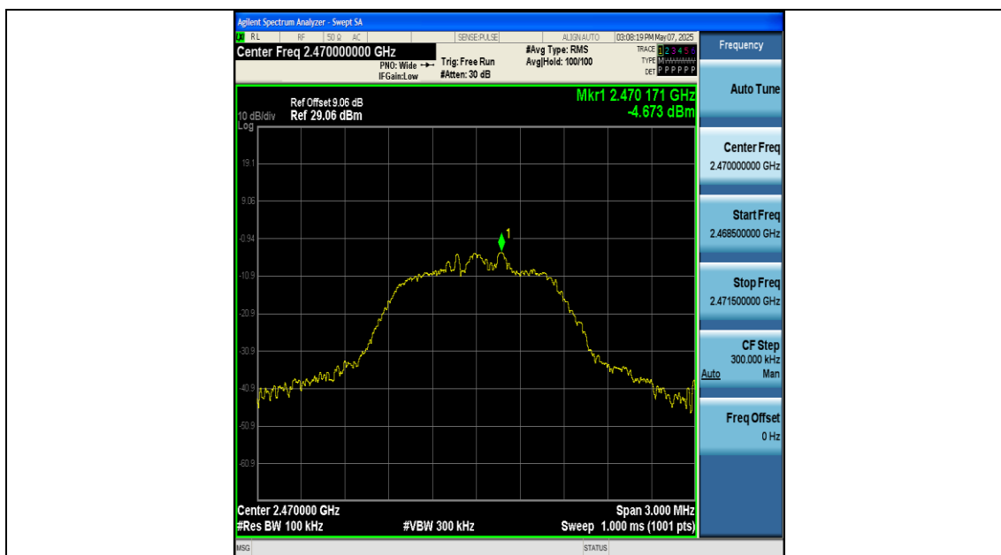
SRD-Ant1-2470-0~Reference-PASS
