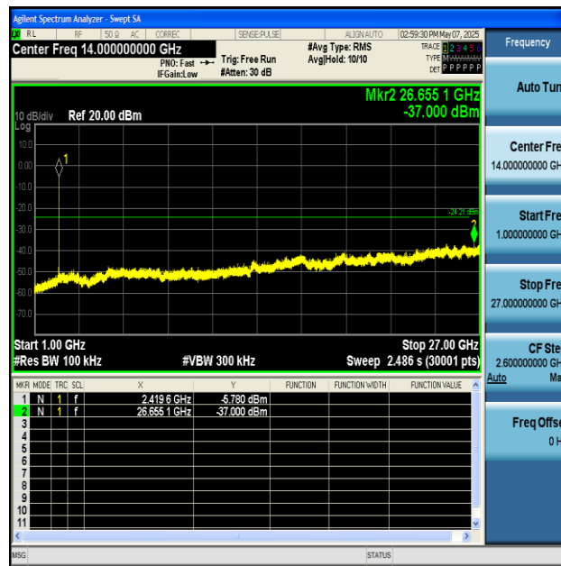
SRD-Ant1-2420-1000~27000-PASS
