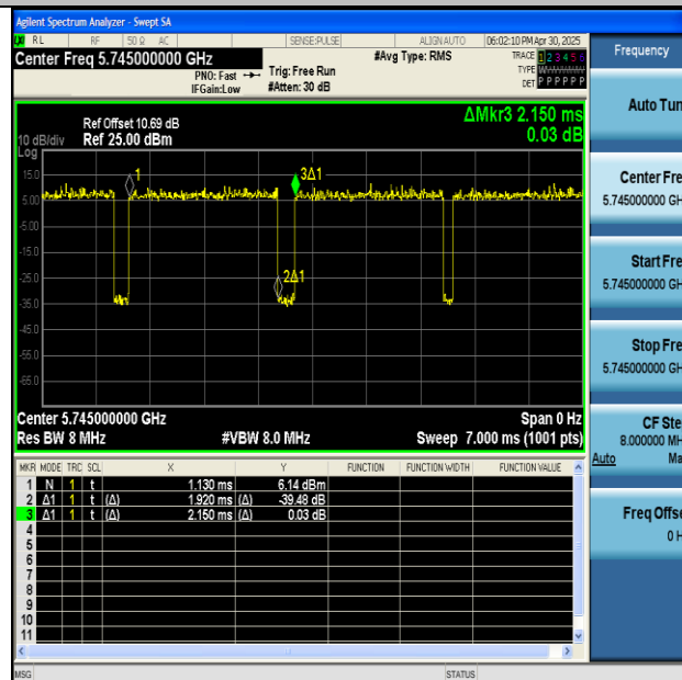
NTNV-11N20SISO-Ant1-5745
