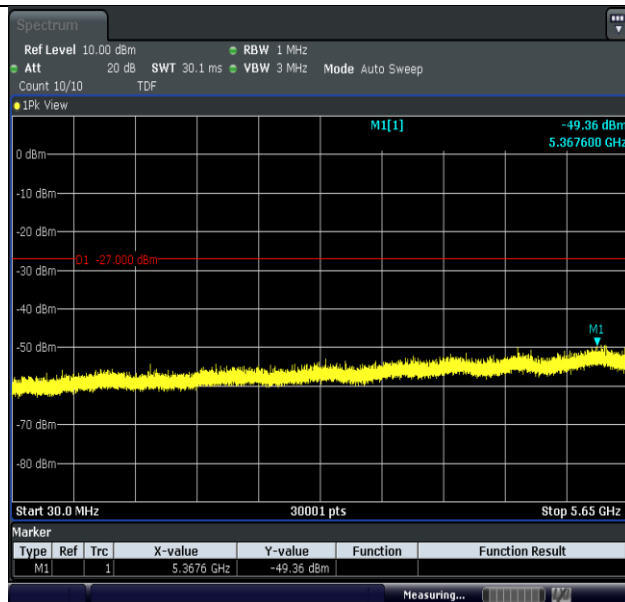
11N20SISO-Ant1-5785-30~5650-PASS
