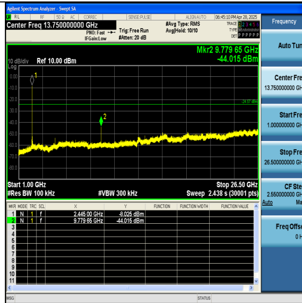
SRD-Ant1-2445-1000~26500-PASS
