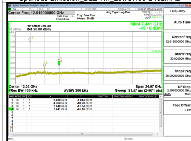
Spurious Emission_BLE 1M_HighCH39-2480MHz
