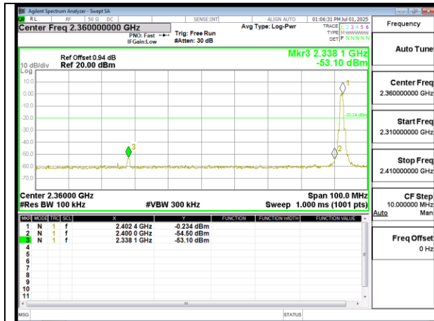
Band Edge_BLE 1M_LowCH00-2402MHz
