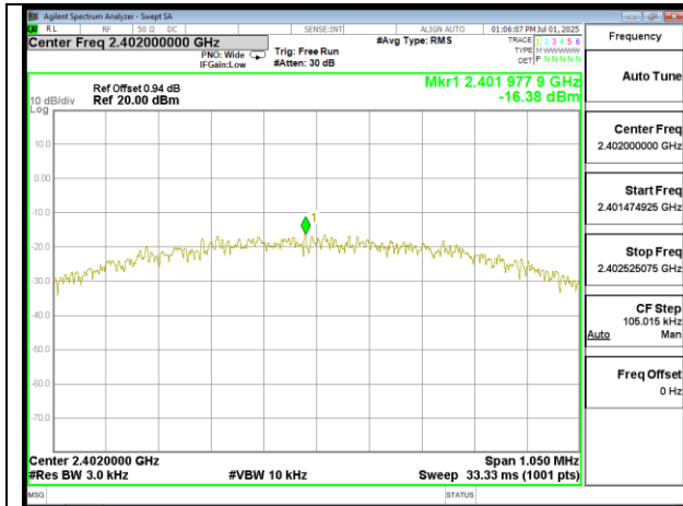
PSD_BLE 1M_LowCH00-2402MHz
