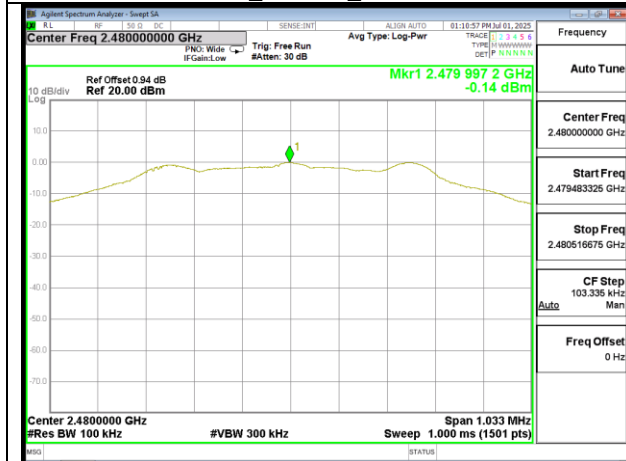
Reference Level_BLE 1M_HighCH39-2480MHz
