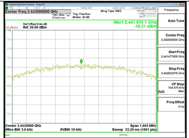
PSD_BLE 1M_MidCH20-2442MHz
