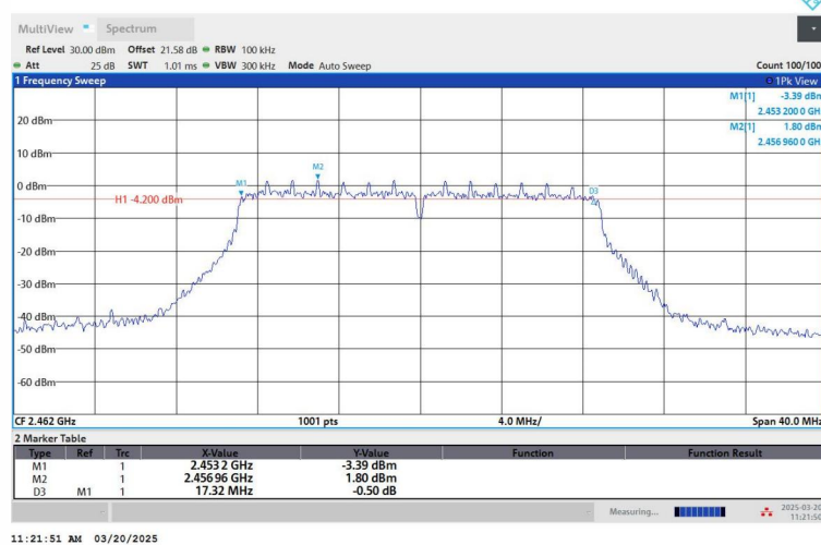
11N20SISO-Ant1-2462
