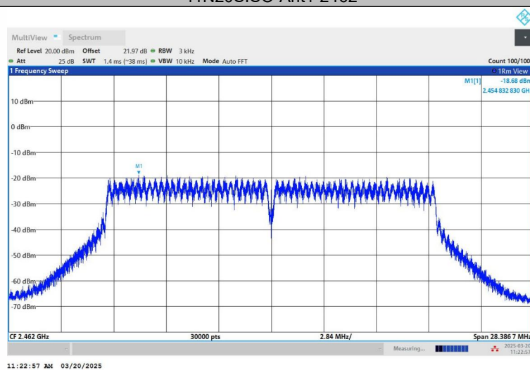
11N20SISO-Ant1-2462
