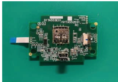
Circuit of wireless (back)
