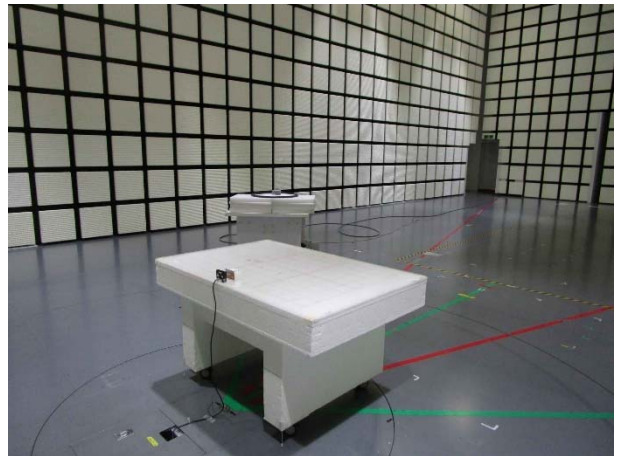
Rear (Loop Antenna: Horizontal)
