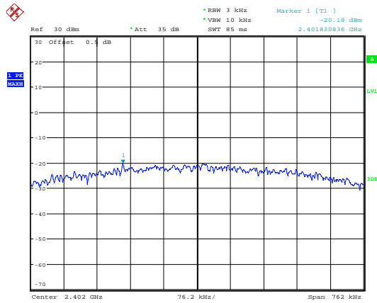
BLE_1M_Low_Channel
