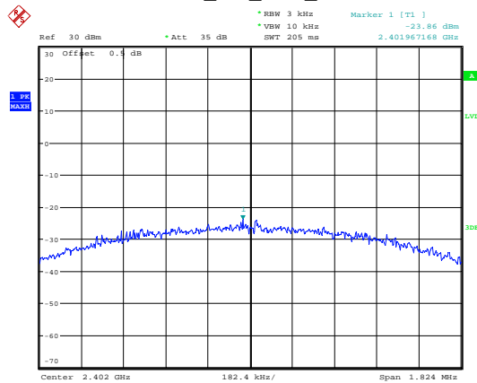
BLE_2M_Low_Channel
