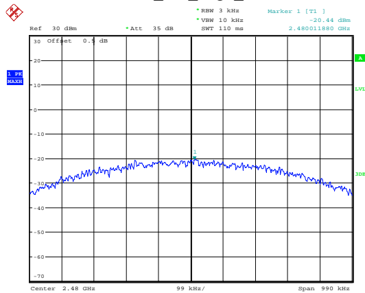
BLE_1M_High_Channel
