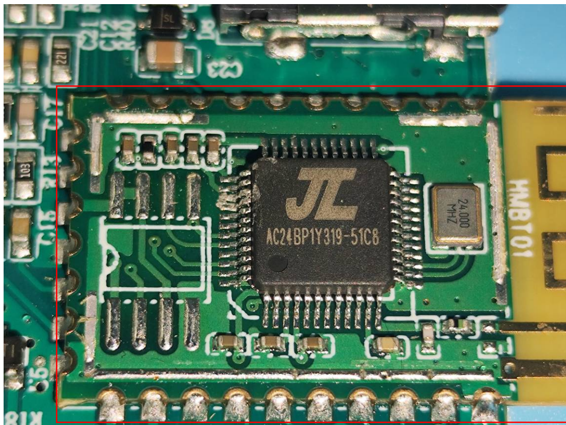
RF Module Unshielded
