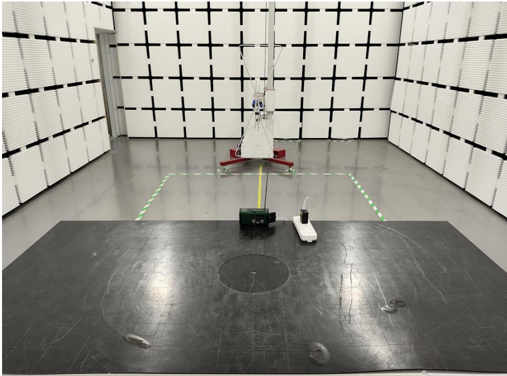
Radiation Emissions Test (<1G)
