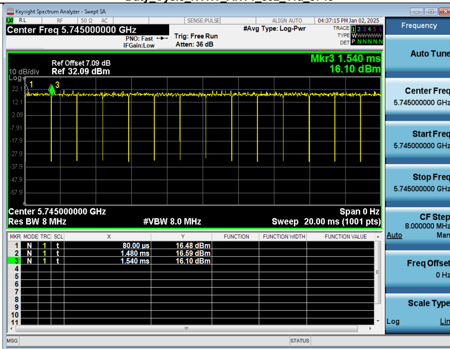
Duty_Cycle_NVNT_ANT2_802_11a_5745
