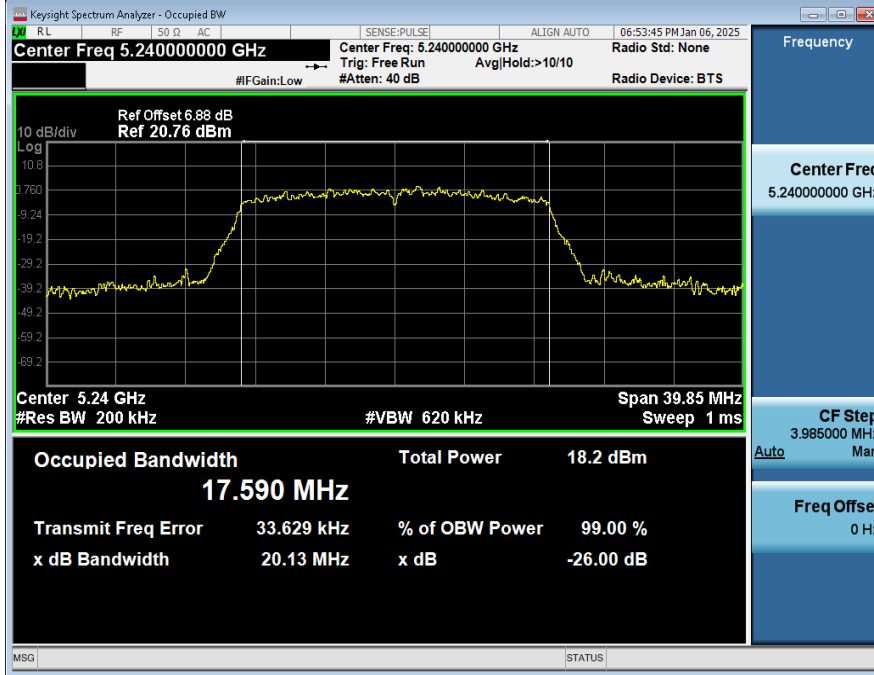
99%_OCB_NVNT_ANT2_802_11ac(VHT20)_5240
