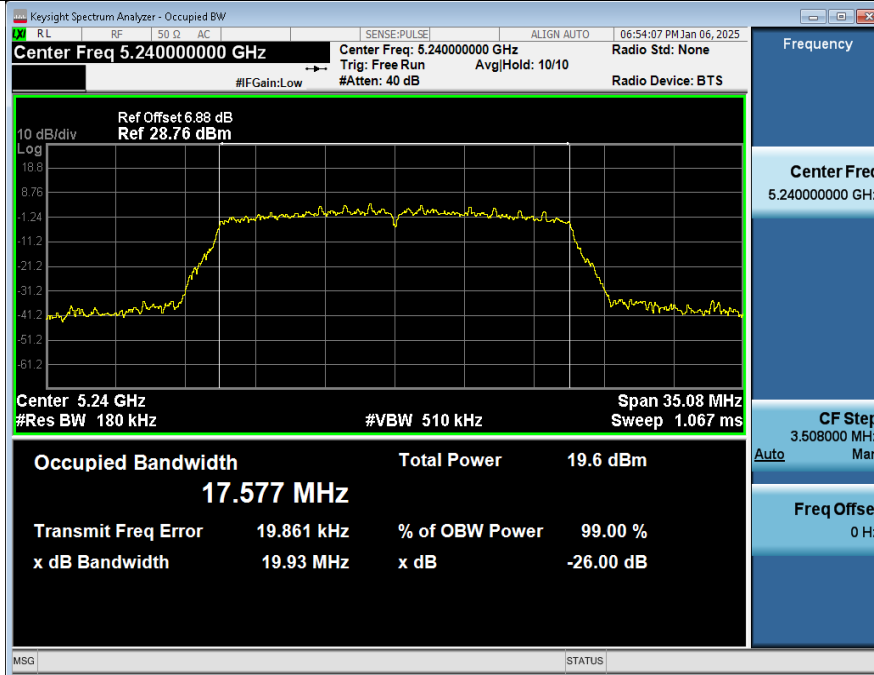
-26BW_NVNT_ANT2_802_11ac(VHT20)_5240
