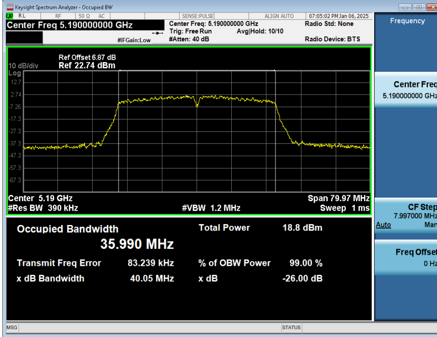
99%_OCB_NVNT_ANT2_802_11n(HT40)_5190
