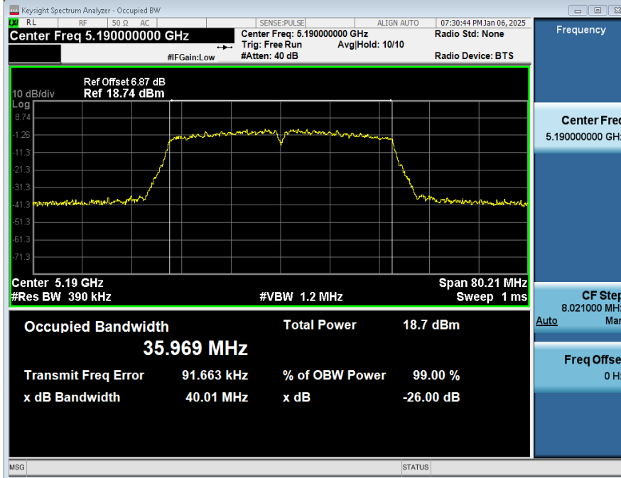
99%_OCB_NVNT_ANT2_802_11ac(VHT40)_5190
