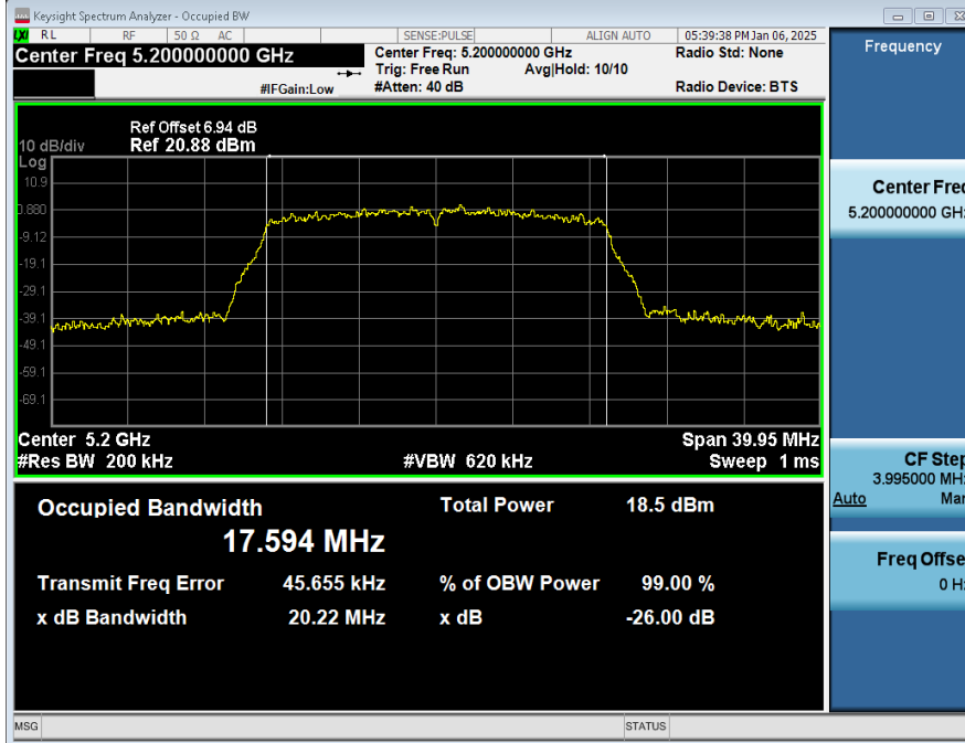
99%_OCB_NVNT_ANT2_802_11n(HT20)_5200
