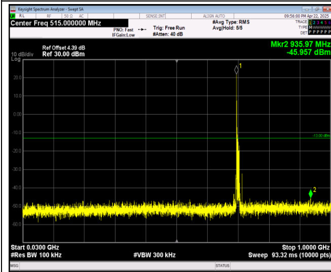
Band12-10MHz-16QAM-23095-1RB#0-Range1:30~-1000MHz
