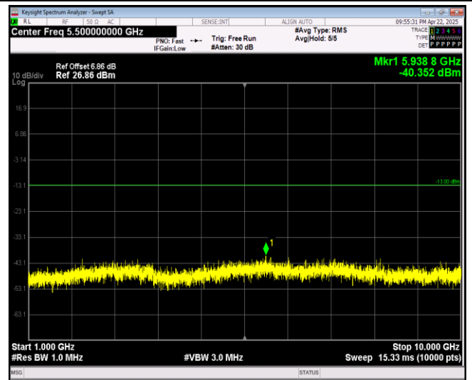
Band12-10MHz-16QAM-23095-1RB#0-Range2:1000~10000MHz
