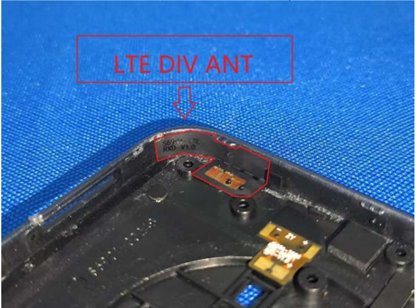
LTE Band7/41 ANT
