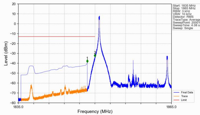
Band25_15MHz_QPSK_LCH_1857.5MHz_RB_1_0_NTNV
