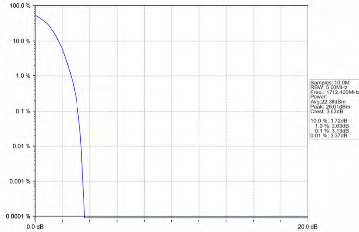
Band4_RMC_LCH_1712.4MHz_12.2kbps RMC_NTNV
