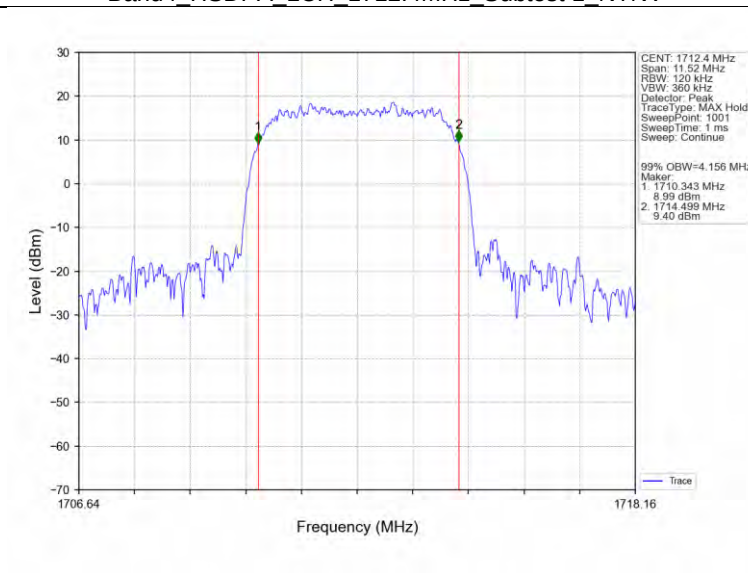
Band4_HSDPA_LCH_1712.4MHz_Subtest 1_NTNV
