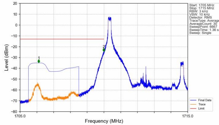
Band66_5MHz_QPSK_LCH_1712.5MHz_RB_1_0_NTNV
