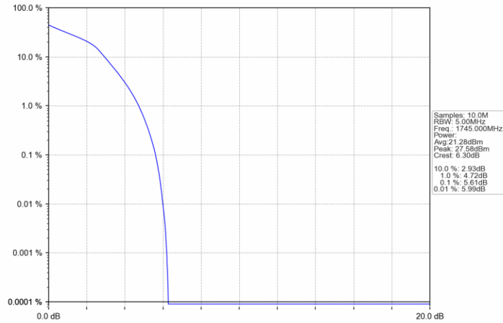
Band66_3MHz_16QAM_MCH_1745MHz_RB_15_0_NTNV
