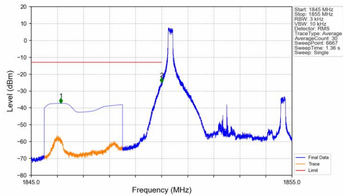
Band25_5MHz_QPSK_LCH_1852.5MHz_RB_1_0_NTNV
