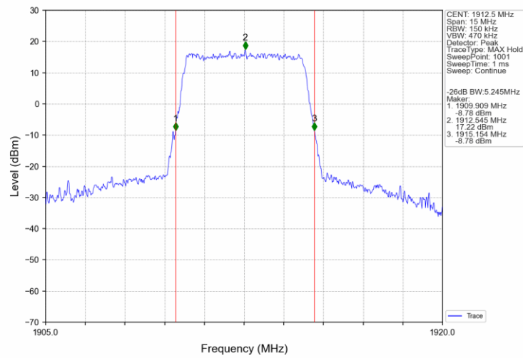
Band25_5MHz_16QAM_HCH_1912.5MHz_RB_25_0_NTNV
