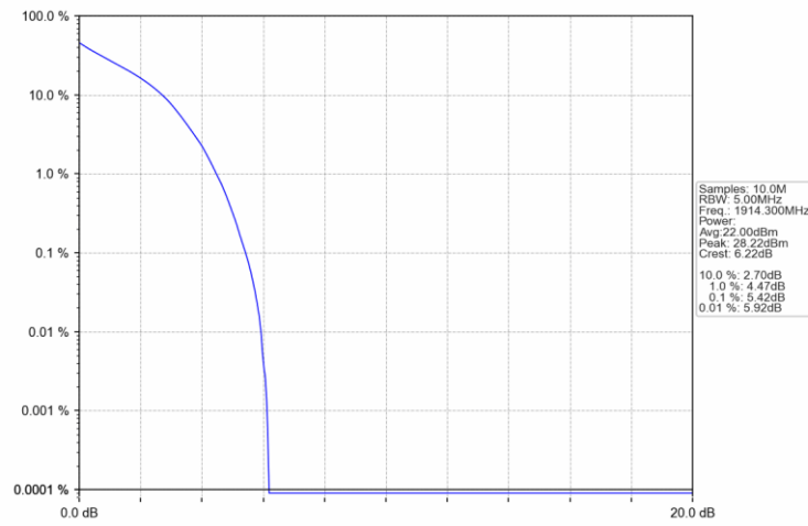
Band25_1.4MHz_QPSK_HCH_1914.3MHz_RB_6_0_NTNV
