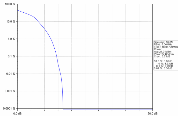
Band25_1.4MHz_16QAM_LCH_1850.7MHz_RB_6_0_NTNV
