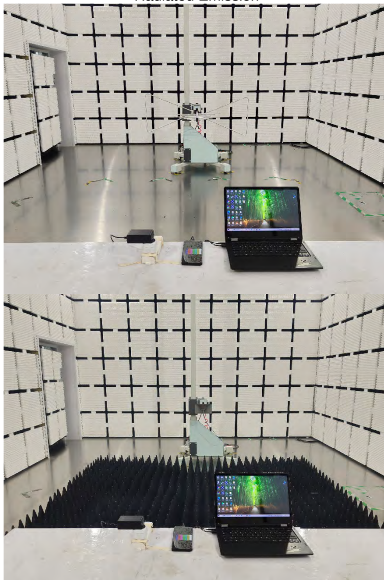
Radiated Emission
