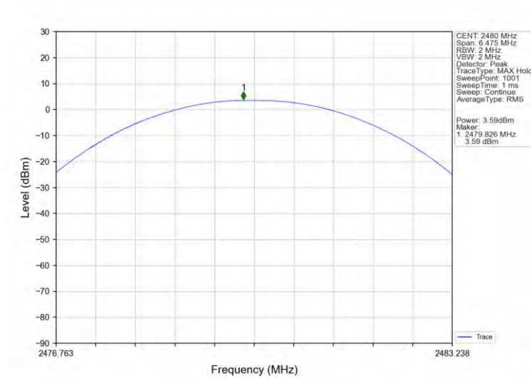
Pi/4DQPSK_2DH5_HCH_2480MHz_Ant1_NTNV
