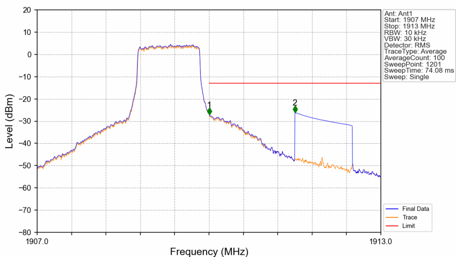
Band2_1.4MHz_16QAM_HCH_1909.3MHz_RB_6_0_NTNV
