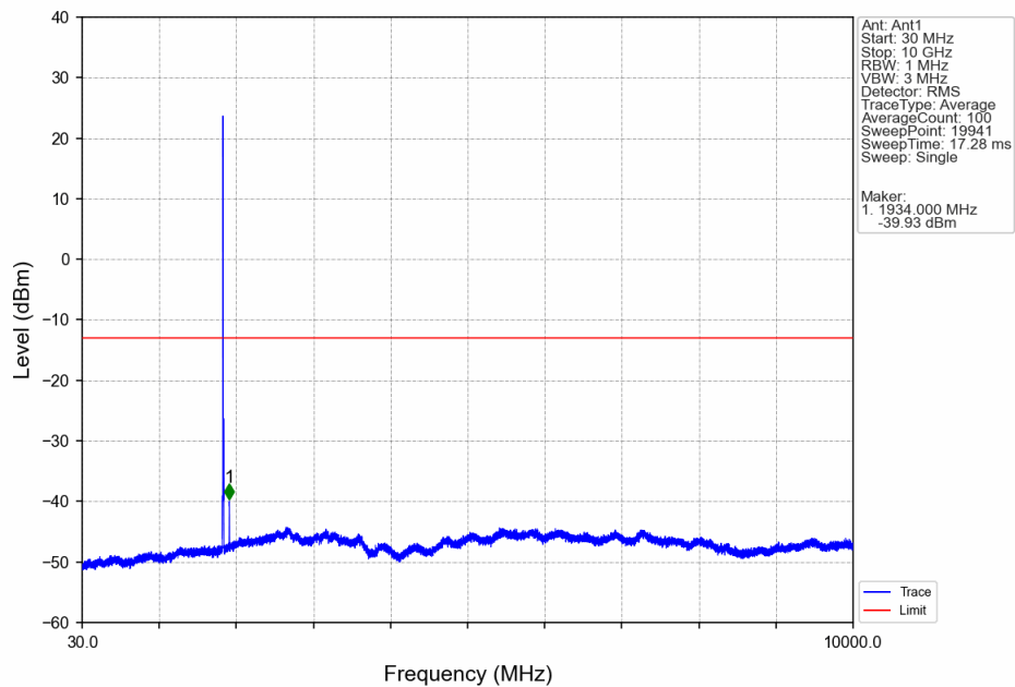
Band2_5MHz_QPSK_LCH_1852.5MHz_RB_1_0_NTNV
