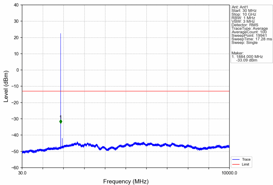
Band2_1.4MHz_16QAM_MCH_1880MHz_RB_1_0_NTNV
