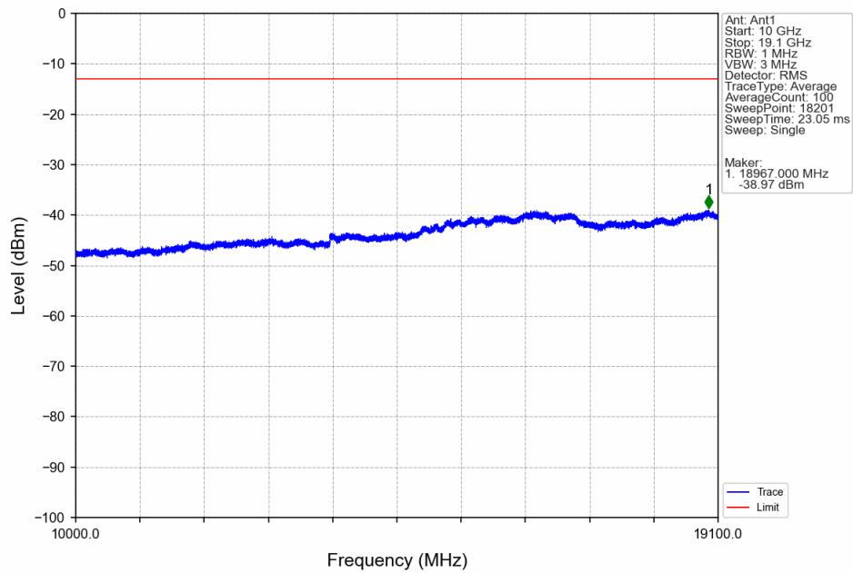
Band2_1.4MHz_QPSK_LCH_1850.7MHz_RB_6_0_NTNV
