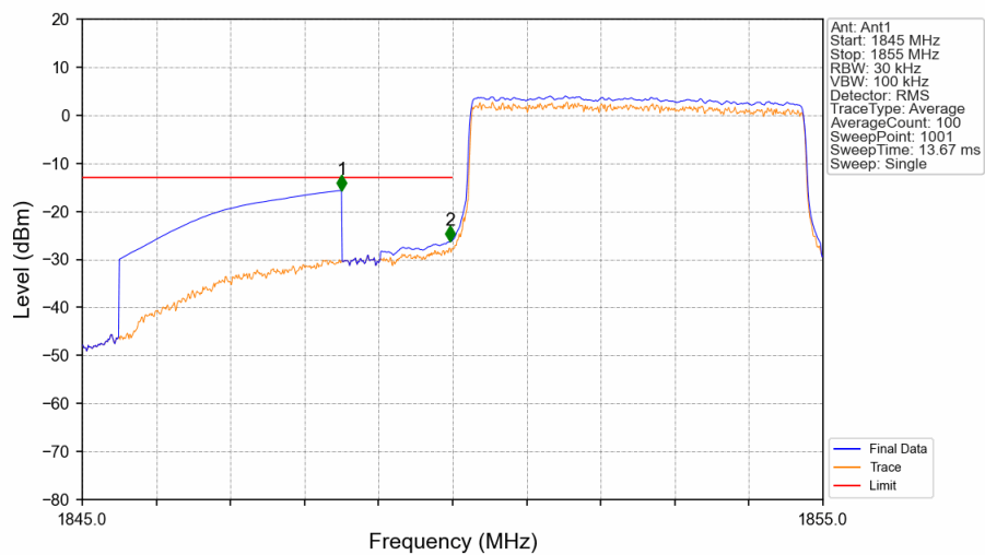
Band2_5MHz_QPSK_LCH_1852.5MHz_RB_25_0_NTNV
