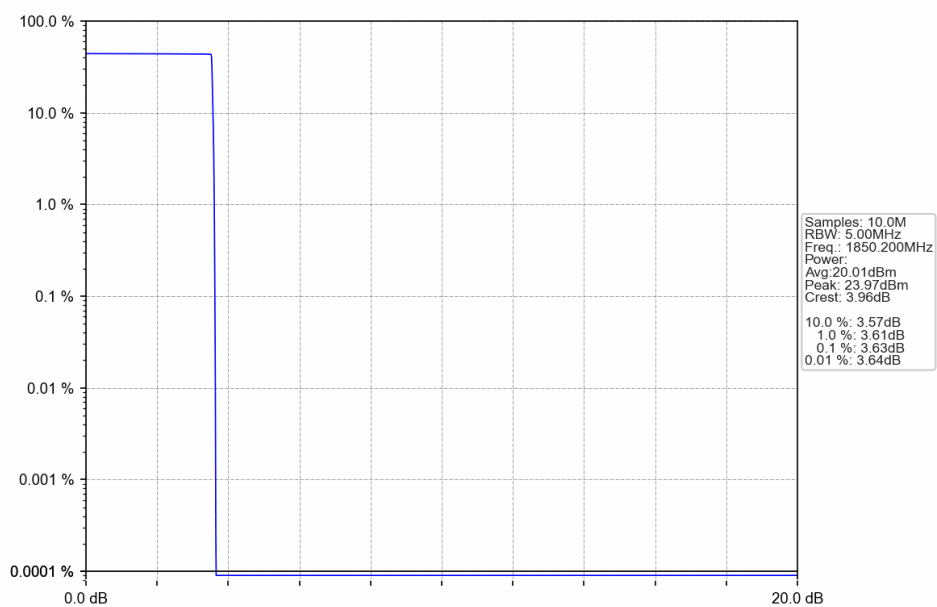
PCS1900 GPRS LCH 1850.2MHz 4 TX Slots NTV
