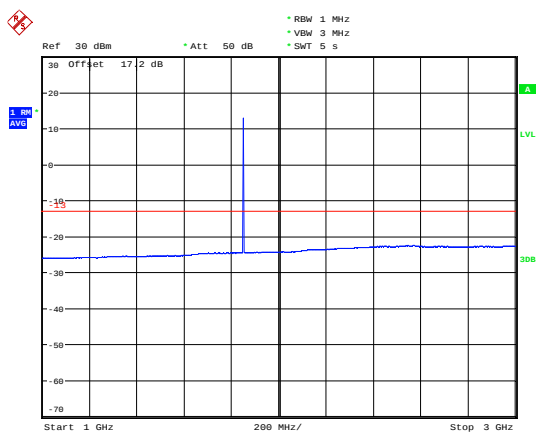
LTE Band 25 5MHz CH-Low 1GHz~3GHz
