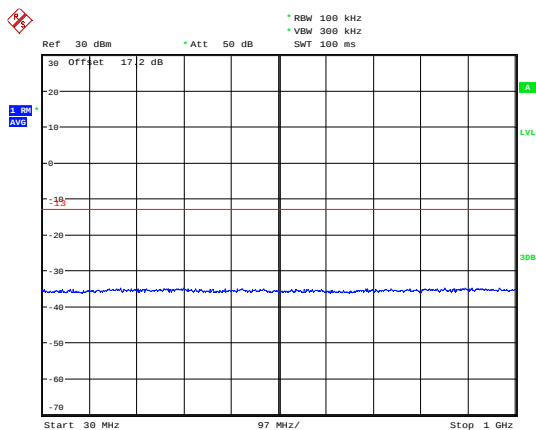
LTE Band 25 5MHz CH-Low 30MHz~1GHz
