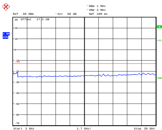
LTE Band 25 5MHz CH-Low 3GHz~20GHz
