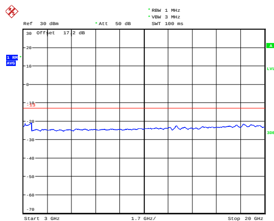
LTE Band 25 5MHz CH-Middle 3GHz~20GHz
