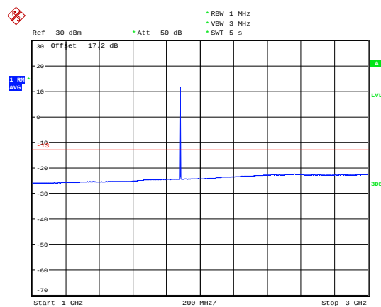
LTE Band 25 5MHz CH-Middle 1GHz~3GHz
