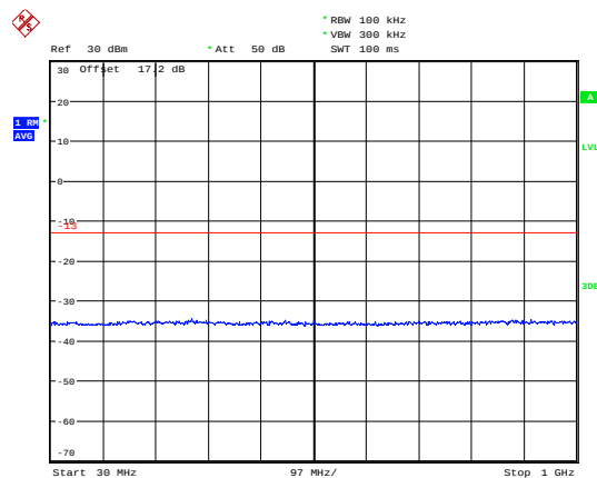
LTE Band 25 5MHz CH-Middle 30MHz~1GHz
