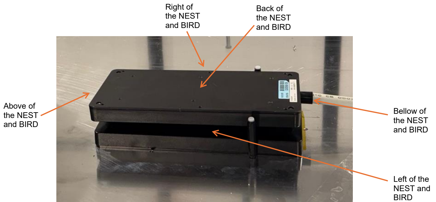
Photo of the test setup – WPT + Bluetooth mode – NEST on top of the BIRD
