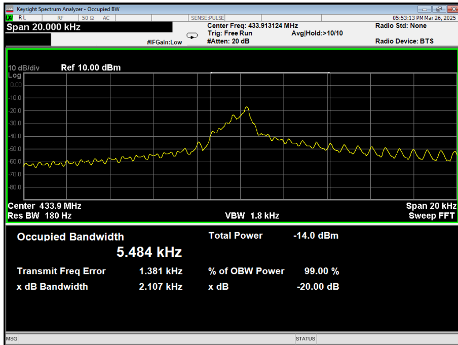
Test Plots of 20dB Bandwidth
