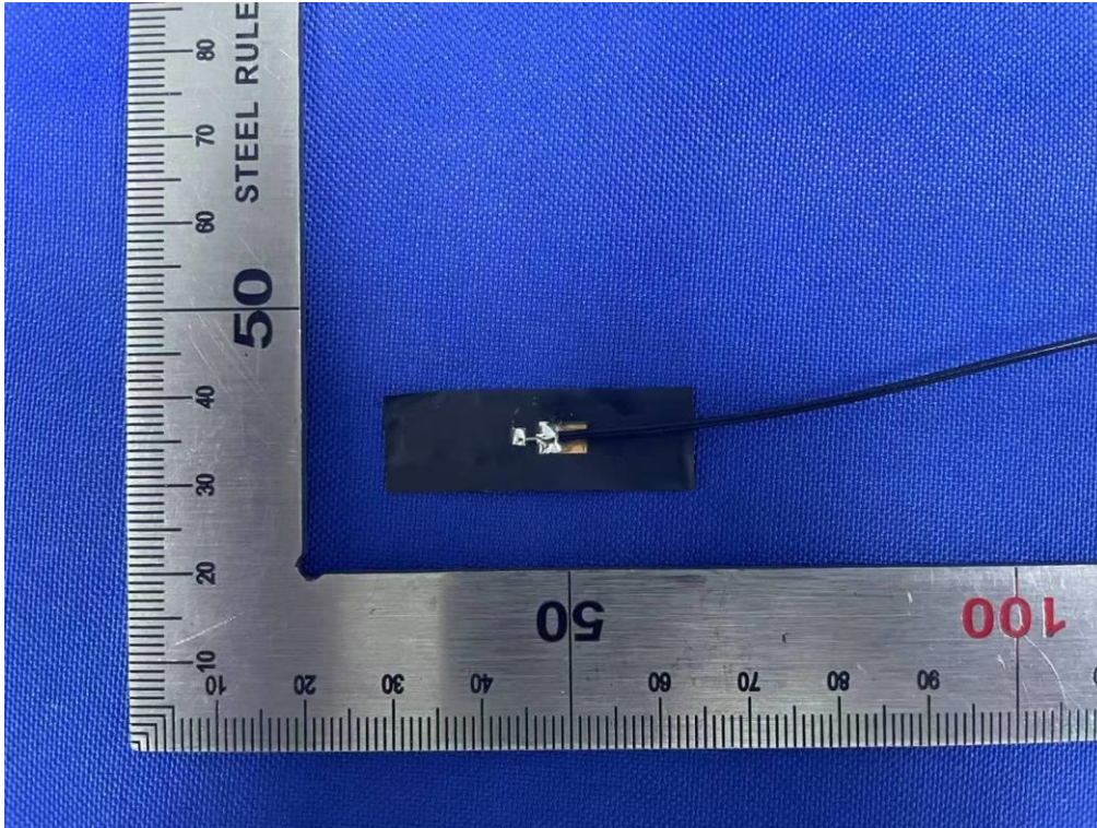
Antenna photo-1
