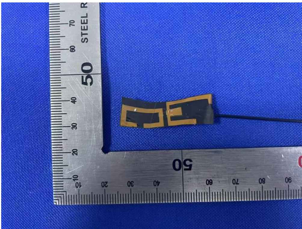
Antenna photo-2
