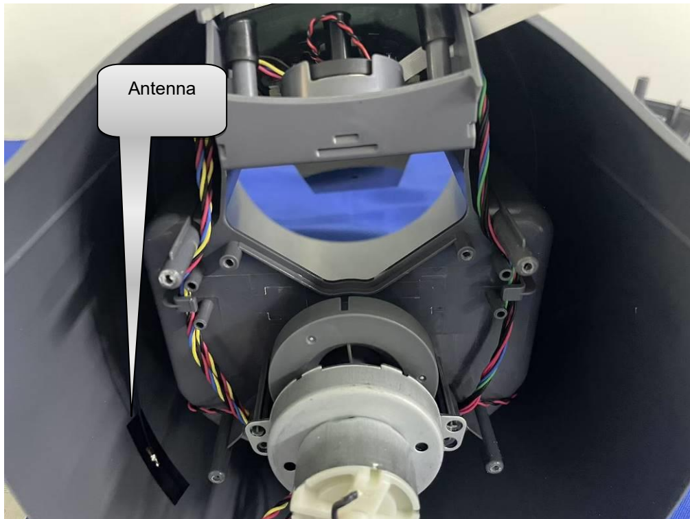
Antenna Position
