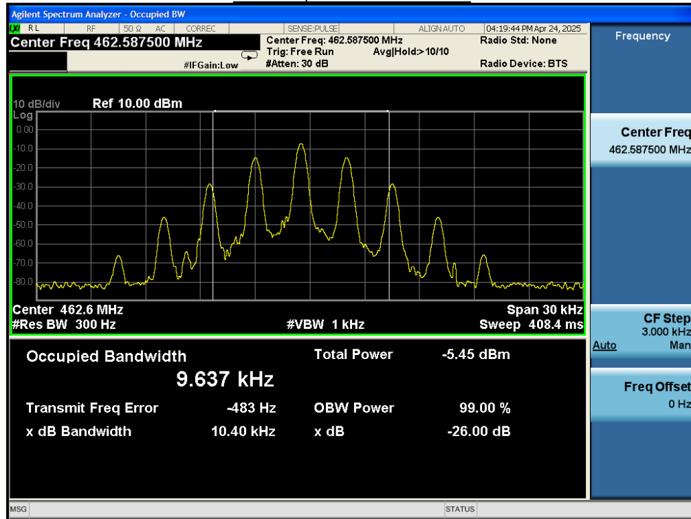
Test Graph for 462.5875MHz
