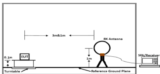
Figure 1. Below 30MHz
