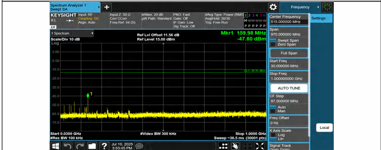
11N20SISO-Ant1-2437-30~1000-PASS
