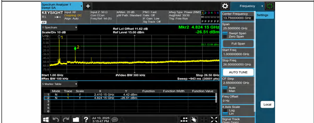
11B-Ant1-2412-1000~26500-PASS
