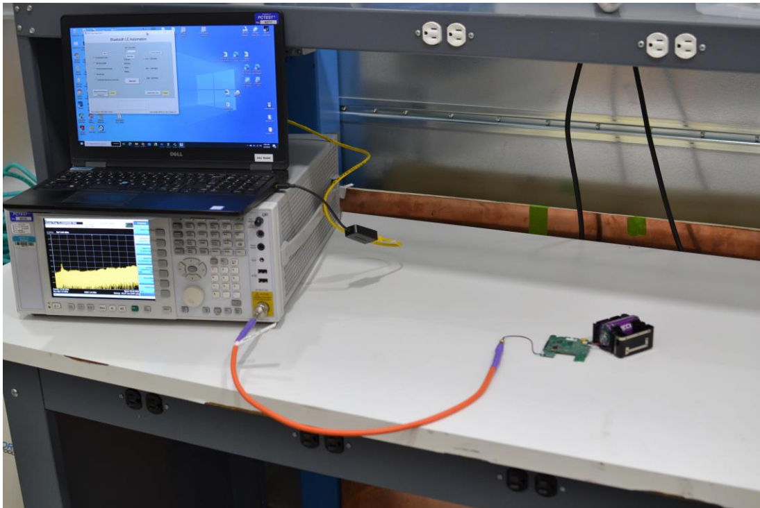
Conducted Emissions
