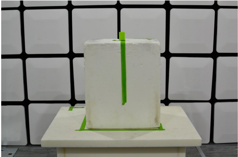
Radiated Emissions Back
